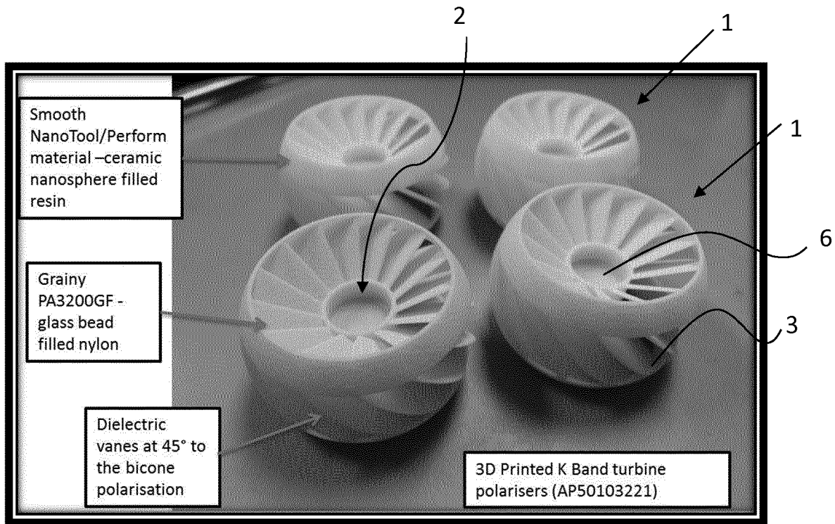
Figure 3: Manufactured 3D printed turbine polarisers, showing each as a single printed piece part.
