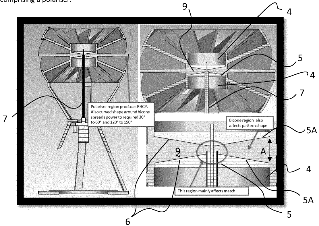
Figure 5: A schematic sectional view of a computer model of one form of the K band antenna comprising a polariser.
