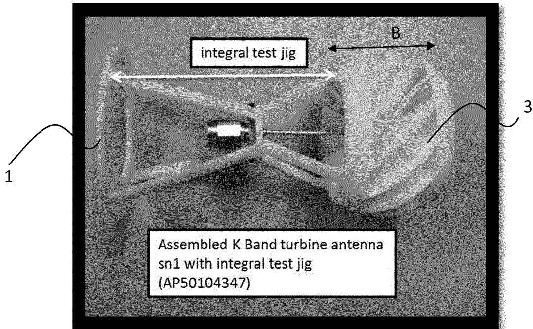
Figure 4: One form of assembled K Band antenna with integral jig is shown below.
