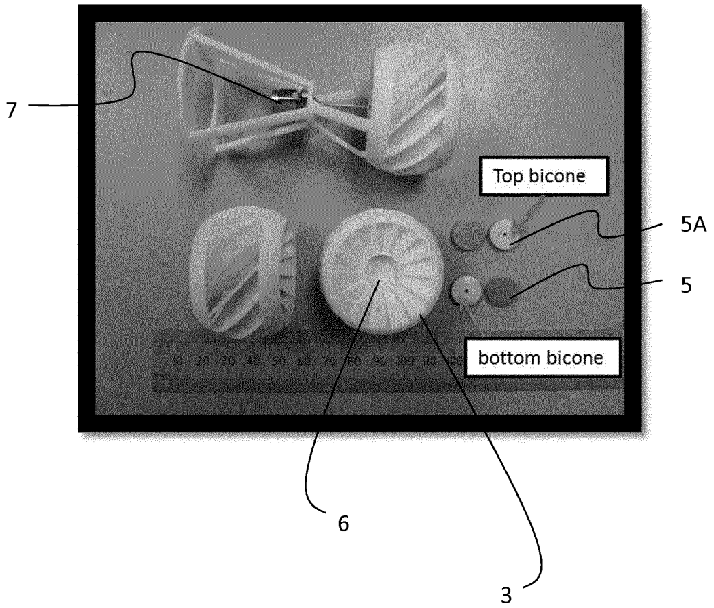
Figure 8: A glass filled nylon turbine polariser in accordance with a further form of the invention.
