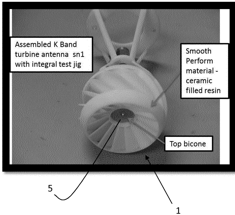
Figure 6: An alternative view of one form of the assembled K Band antenna in accordance with the invention.
