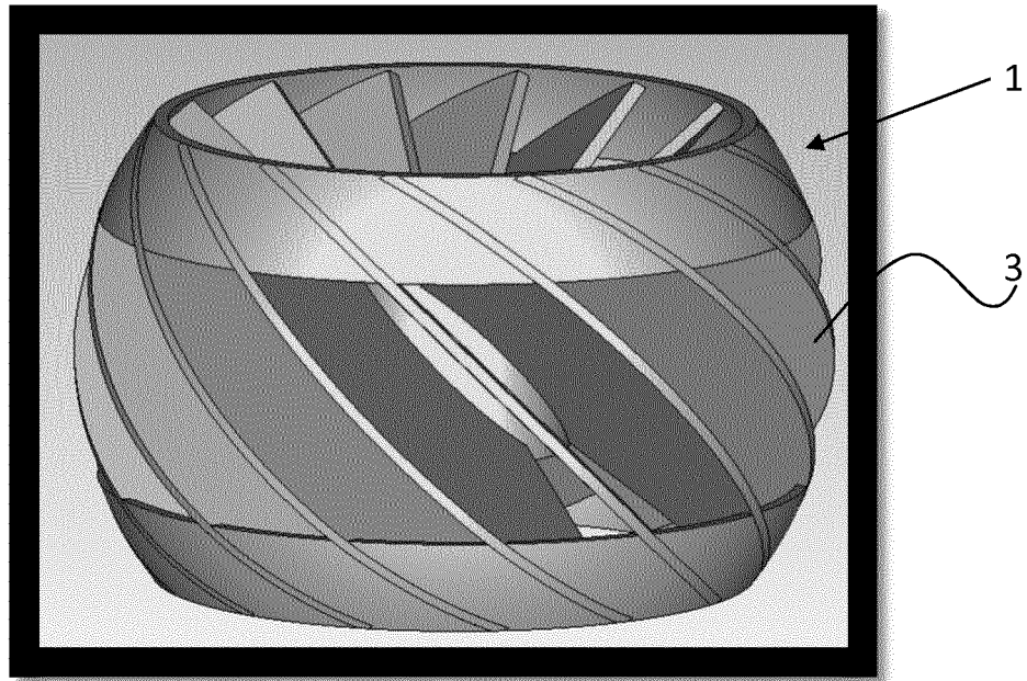
Figure 2: A computer model of the single piece part plastic turbine polariser is shown below.
