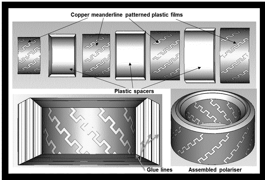
Figure 1: A cylindrical meanderline polariser
