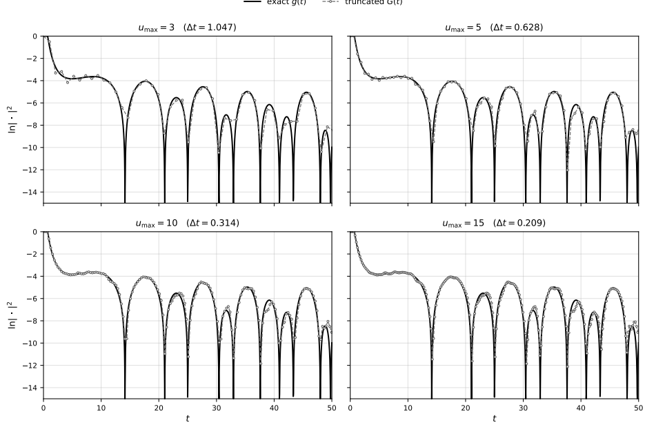
Figure 3: Effect of truncating and sampling the van der Pol aperture. The solid curve is the exact quantity \ln|g(t)|^2 from Equation (3); dashed curves with markers show \ln|G(t)|^2 computed directly from Equation (4) with du = 0.01 at the natural discrete Fourier spacings \Delta t = 2\pi/(2u_{\max}) . Increasing u_{\max} gives finer Fourier sampling and closer reproduction of the exact zero structure.
